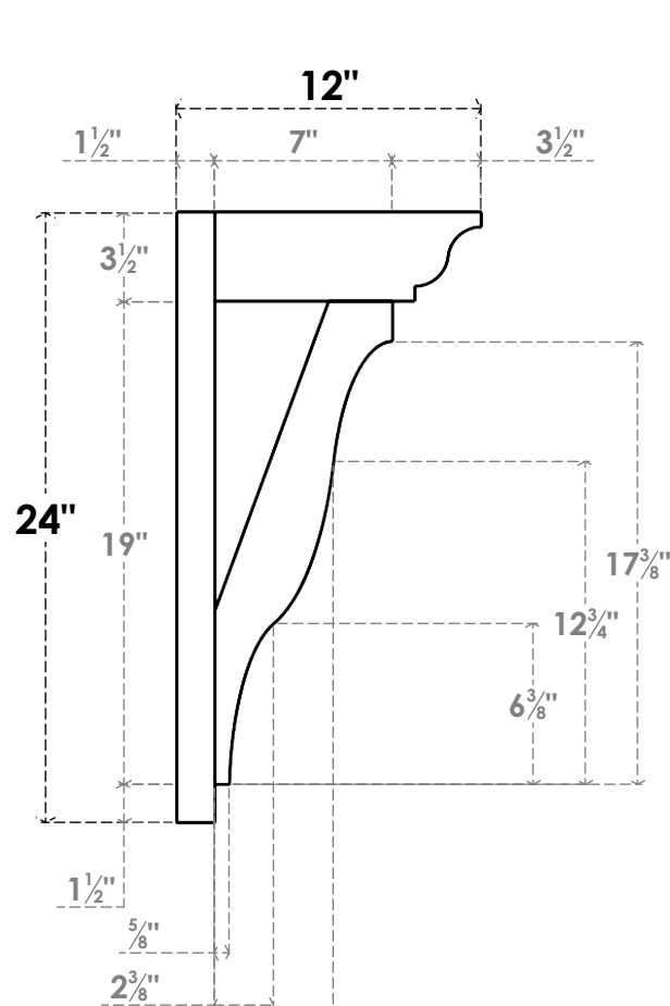
SIDE PROFILE
